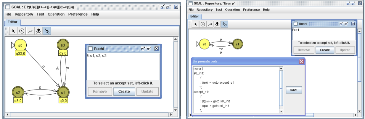
(a) Automaton translated from the QPTL formula
